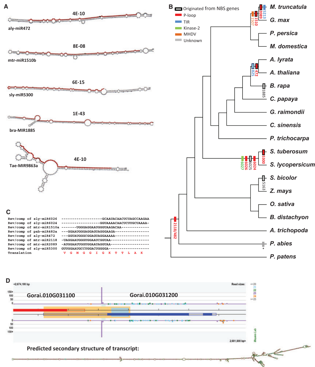
FIG. 3. Convergent evolution of miRNA-targeting NBS-LRRs. (A) Some miRNA precursors have extended similarity with NBS genes beyond miRNAs. The red highlighted sequence represents a miRNA precursor with a best BLAST hit to an NBS gene. The number above the hairpin is the e -value of the best BLAST hit. (B) MicroRNAs continuously emerged during the evolution of higher plants and target encoded, conserved motifs of NBS proteins. The boxes represent the birth of a miRNA during the differentiation of plant ancestors, as determined from the earliest lineage in which it was identified. Boxes with a black outline indicate miRNAs with evidence of origination from an inverted repeat of an NBS gene. Red, blue, orange, and green miRNAs target the encoded P-loop, TIR, Kinase-2, or MHDV motif of NBS genes, respectively. The asterisk for spruce indicates many diverse miRNAs target NBS-LRRs (Xia et al. 2015). All the red identifiers indicate separate origins of miRNAs that target the same P-loop-encoding region of NBS-LRRs. (C) Alignment of reverse-complement of the sequence of miRNAs targeting NBS genes, indicating their target sites around the encoded P-loop motif (the amino acids for this are shown at the bottom). (D) Above, a potential siRNA-producing locus formed by two inverted repeats of a homogeneous NBS-LRR gene pair. The red and blue bars indicate two annotated NBS genes as a convergent pair in the cotton genome. The orange box indicates a predicted inverted repeat. The small dots illustrate 21–24-nt small RNAs in the region (according to the legend in the upper right). Below, the MFE secondary structure of the inverted repeat was predicted by RNAfold.
